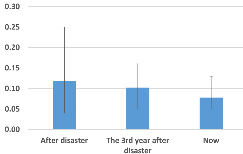
Change of Radiation in Aizu area
